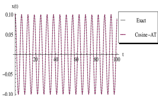
Figure 2: Comparison of the approximate periodic solution, Eq. (32), using CAT technique and the exact solution for the Duffing equation at \epsilon=0.1 and a=0.1 .
